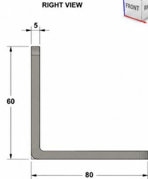
RIGHT VIEW
